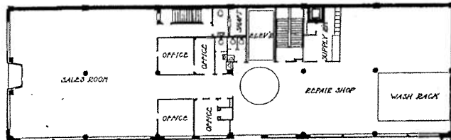
FIRST FLOOR PLAN SCALE 1/8" = 1'-0"
